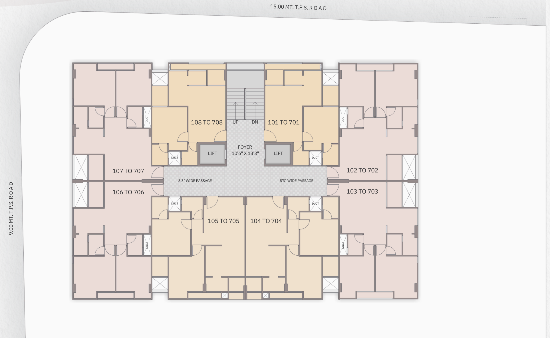
TYPICAL FLOOR PLAN 1ST TO 7TH FLOOR
